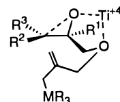
FIGURE 2. Chelated intermediate for \text{TiCl}_4 -promoted allylmetallic cyclization
